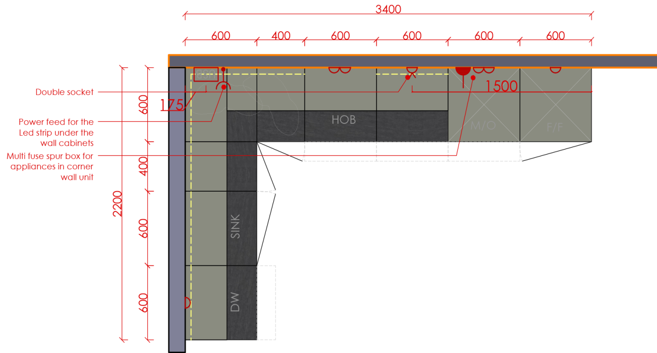
1 PLAN VIEW 1:50 KITCHEN - FLAT TYPE A-05 (FLAT NR.)
